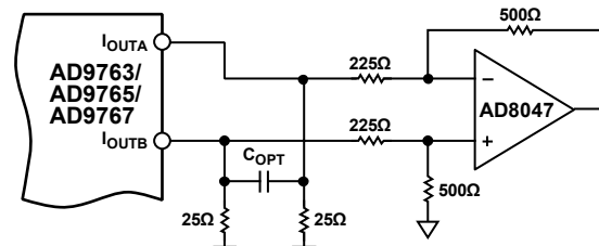
Figure 73. DC Differential Coupling Using an Op Amp
